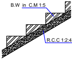
STAIRCASE
