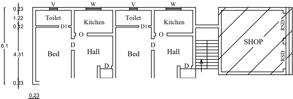
FLOOR PLAN
