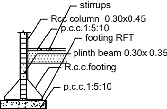
SECTION AB
