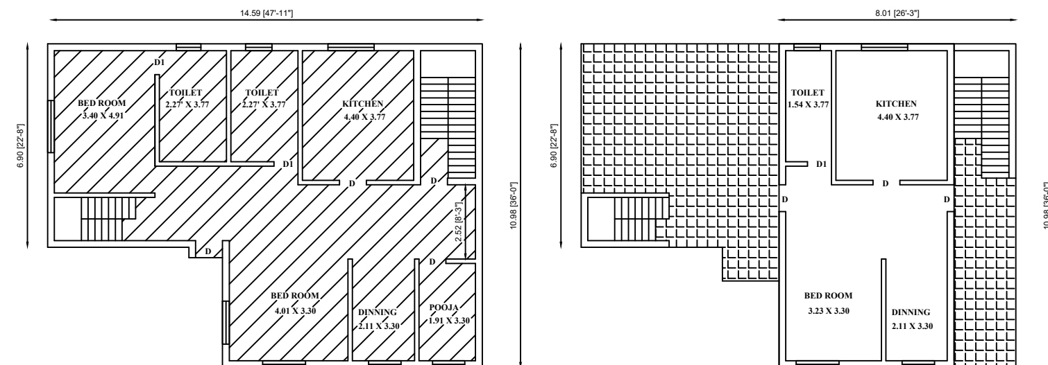
EXG GROUND FLOOR PLAN
