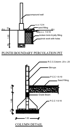
COLUMN DETAIL
