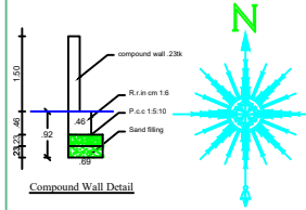
Compound Wall Detail
