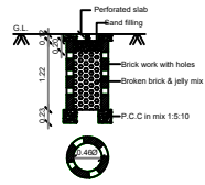
PERCOLATION PIT FOR 30 Sq. m. (Scale:- 1:50)
