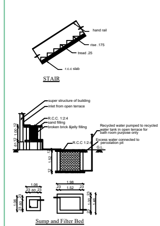
Sump and Filter Bed
