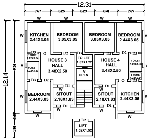
PROPOSED SECOND FLOOR PLAN
