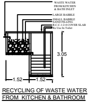
RECYCLING OF WASTE WATER FROM KITCHEN & BATHROOM
