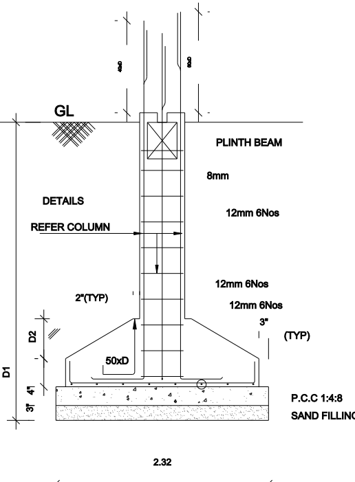
FOUNDATION DETAILS SCALE : 1:50.
