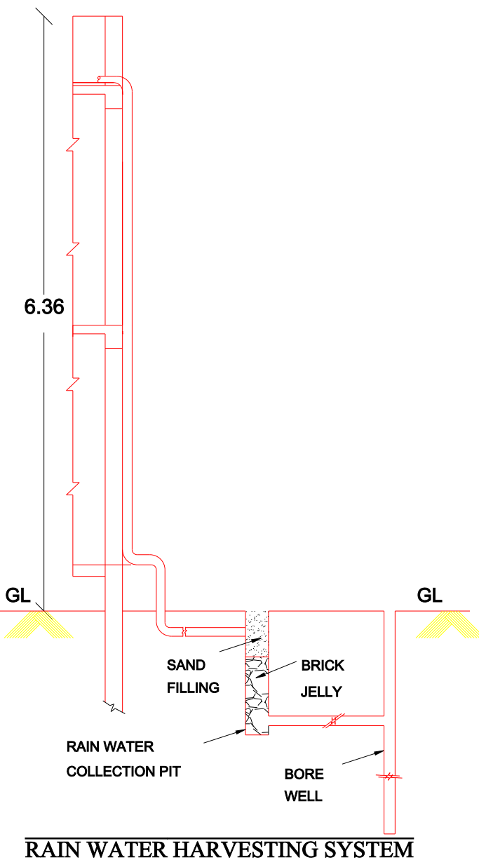
RAIN WATER HARVESTING SYSTEM
