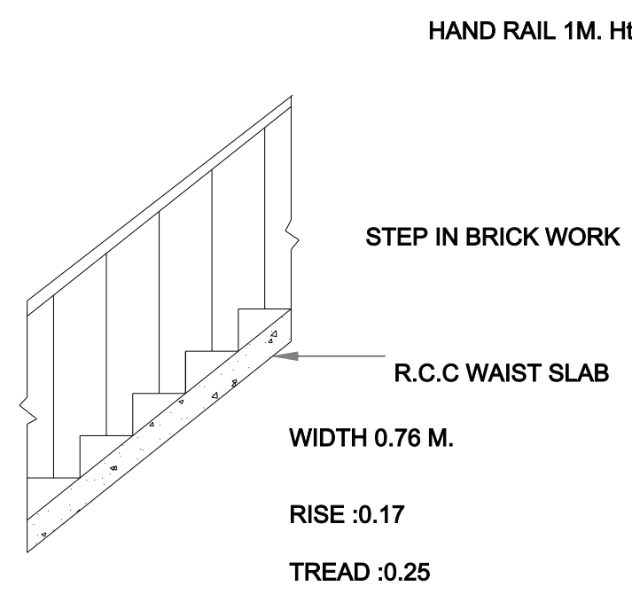
HAND RAIL 1M. HL. STEP IN BRICK WORK R.C.C WAIST SLAB WIDTH 0.78 M. RISE :0.17 TREAD :0.25
