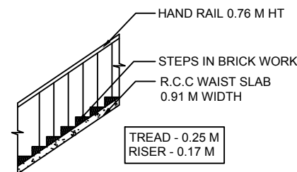
STEP DETAILS
