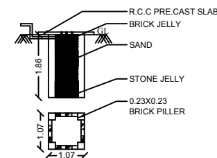
PLAN AND SECTION OF RAINWATER COLLECTION WELL
