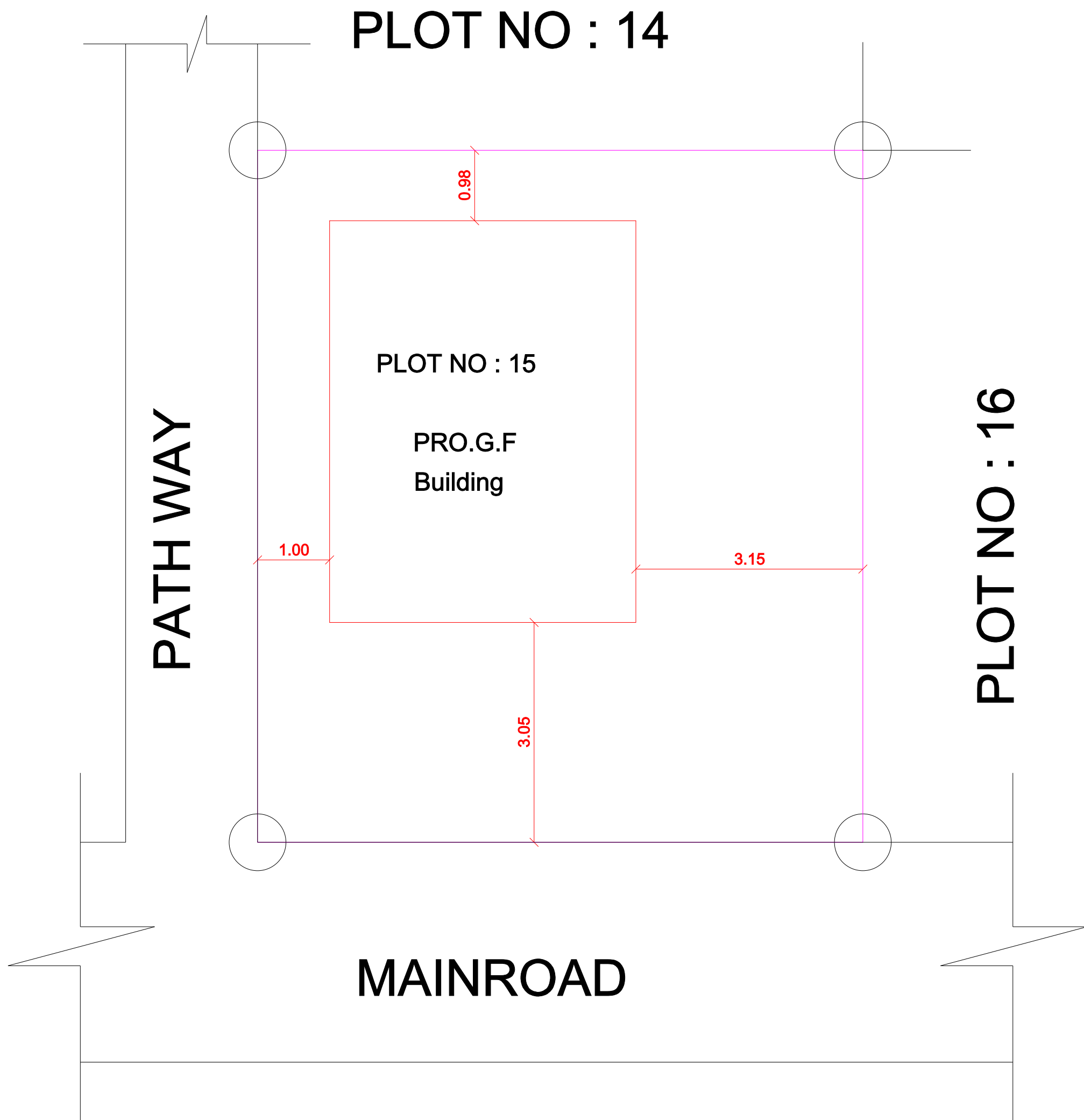
SITE PLAN
