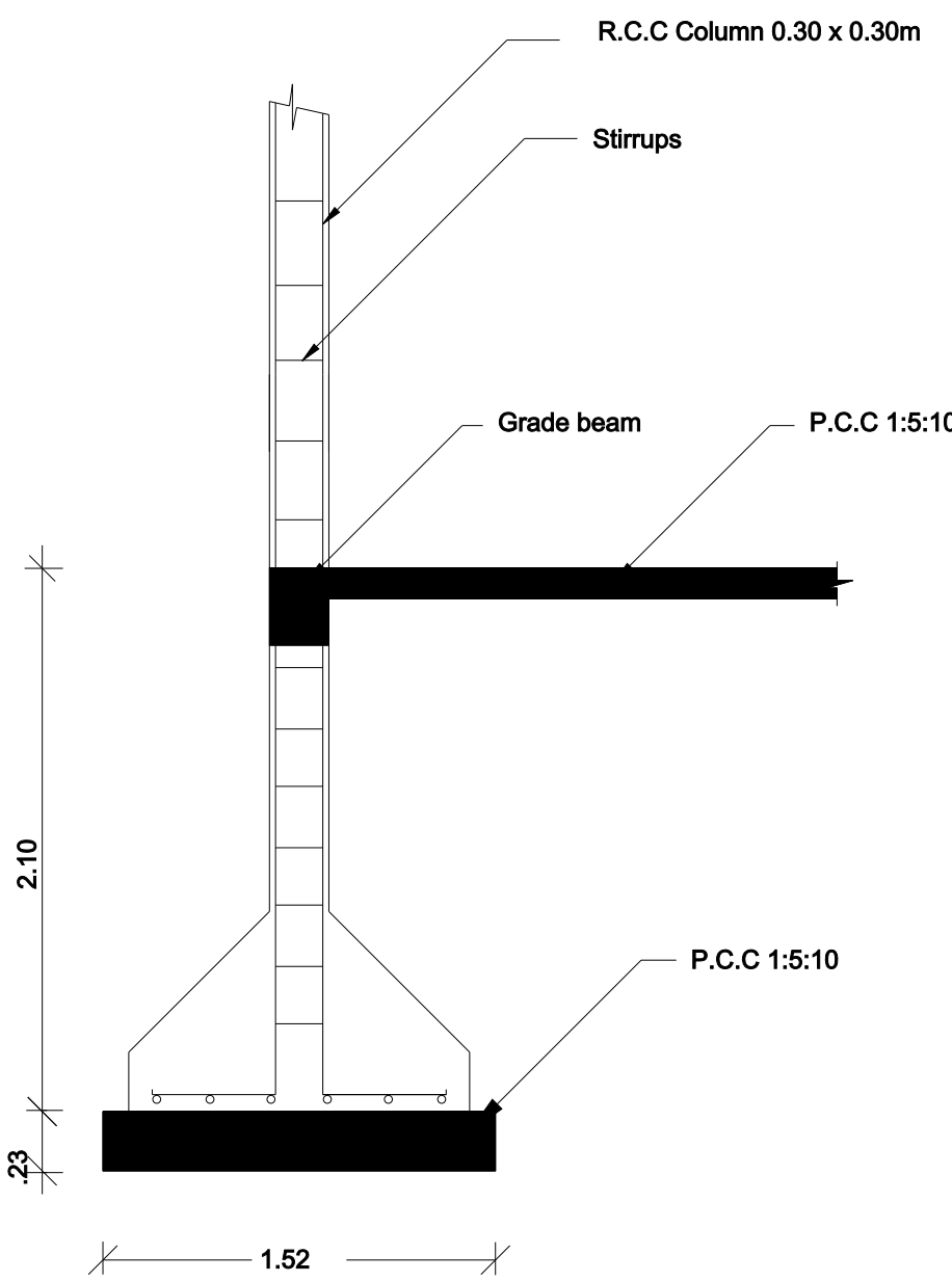
Column Detail
