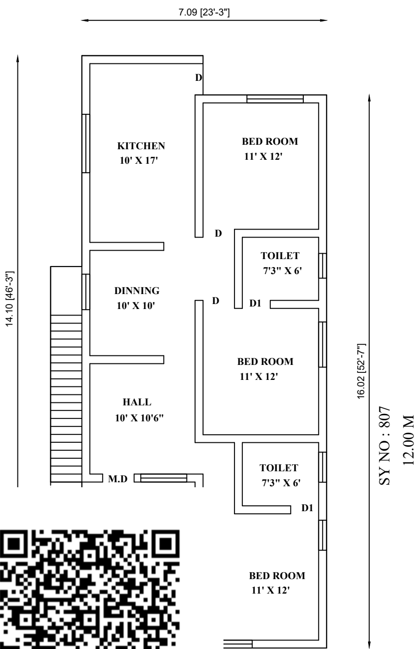
FLOOR PLAN-1
