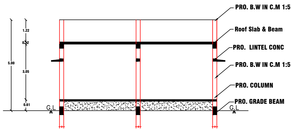
CROSS SECTION ON XX
