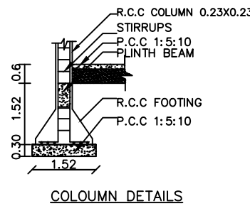
COLOUMN DETAILS
