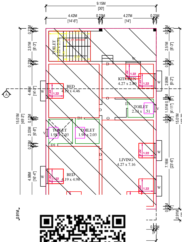
PLAN
