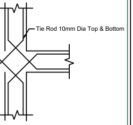
Sectional Plan Beam VS Beam NOT FOR SCALE
