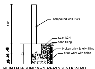
PLINTH BOUNDARY PERCOLATION PIT SCALE (1:50)
