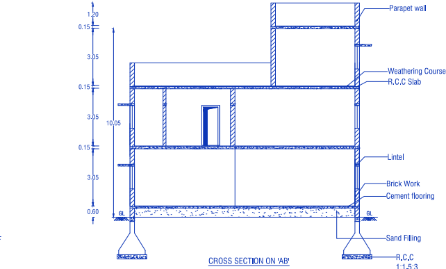
CROSS SECTION ON 'AB'
