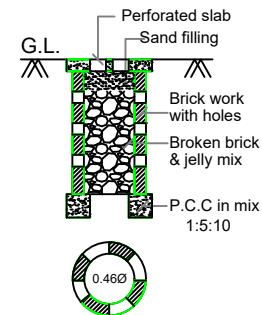
PERCOLATION PIT (NOT FOR SCALE)
