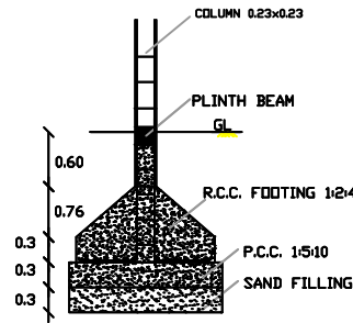
COLUMN DETAILS
