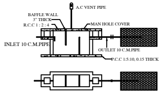
SEPTIC TANK & TRENCH
