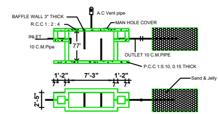
Septic tank and trench
