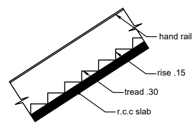
STAIR
