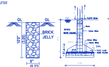
PERCOLATION PIT
