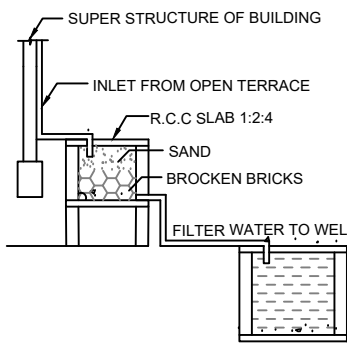
DETAILS OF FILTER BED & WELL
