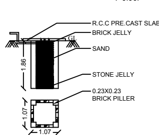
PLAN AND SECTION OF RAINWATER COLLECTION WELL
