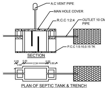
PLAN OF SEPTIC TANK & TRENCH
