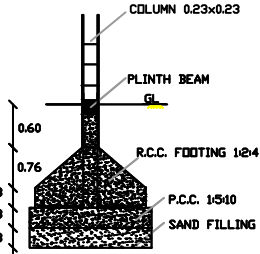
COLUMN DETAILS
