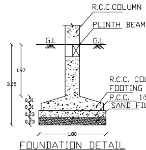
FOUNDATION DETAIL
