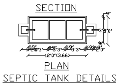
SEPTIC TANK DETAILS
