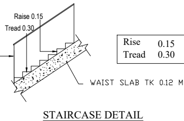
STAIRCASE DETAIL
