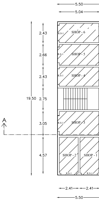
EXISTING GROUND FLOOR APPROVED PLAN
