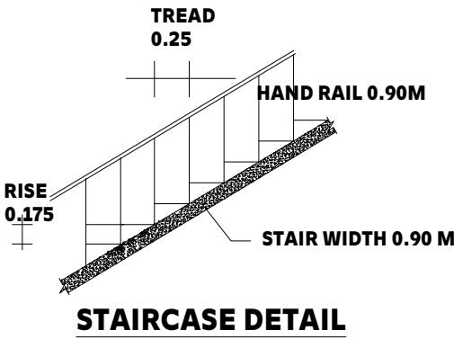
STAIRCASE DETAIL
