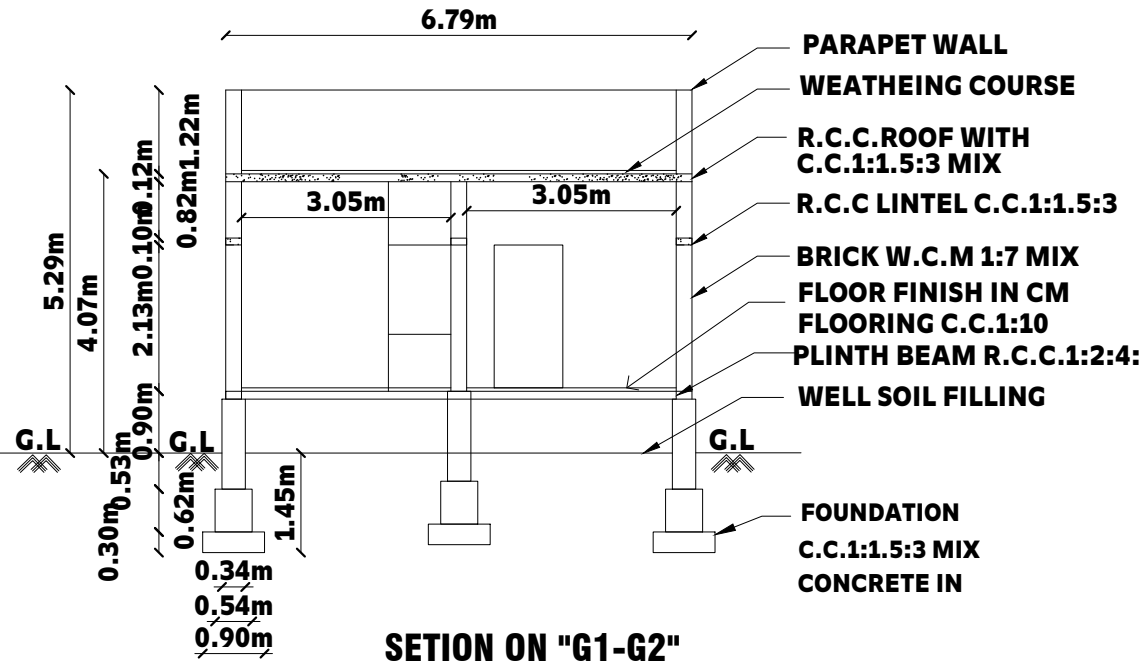
SECTION ON "G1-G2"
