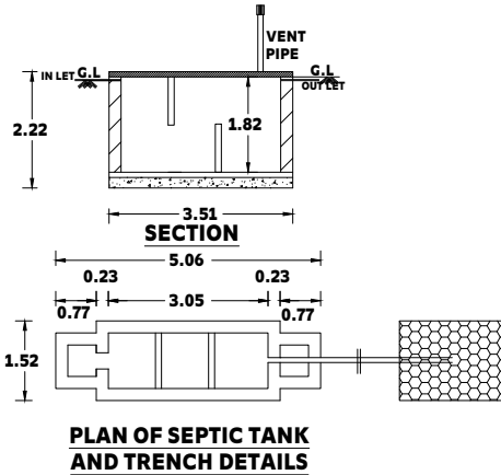
PLAN OF SEPTIC TANK AND TRENCH DETAILS
