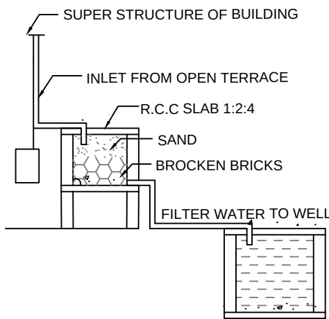
DETAILS OF FILTER BED & WELL
