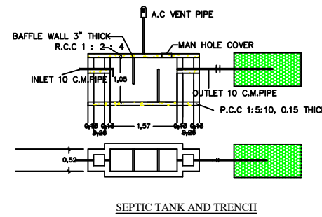
Septic Tank
