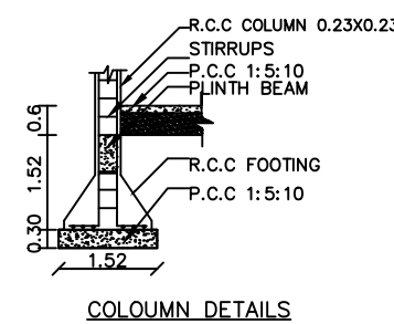
COLOUMN DETAILS
