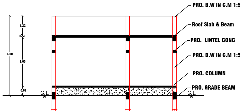
CROSS SECTION ON XX
