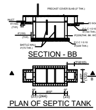
SECTION - BB PLAN OF SEPTIC TANK
