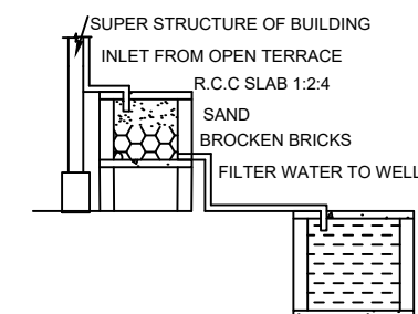
RAINWATER HARVESTING
