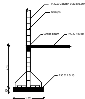
COLUMN DETAIL
