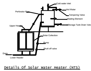
Details of Solar Water Heater (NTS)
