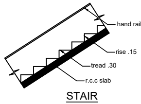
STAIR
