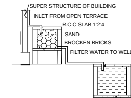
Rainwater harvesting
