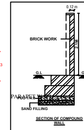
SECTION OF COMPOUND WALL
