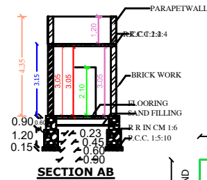
SECTION AB
