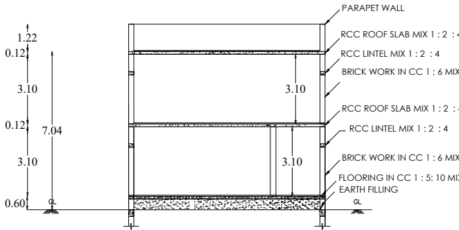
SECTION ON AB & ( HALF ELEVATION)
