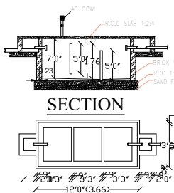
SECTION PLAN SEPTIC TANK DETAILS
