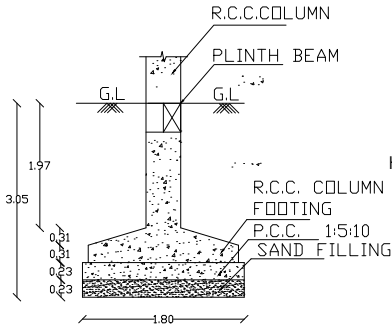
FOUNDATION DETAIL
