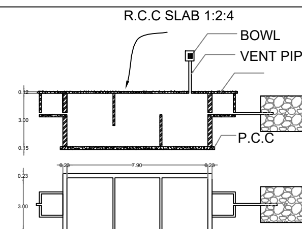
SEPTIC TANK AND TRENCH NTS
