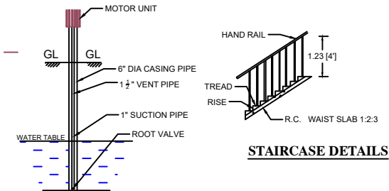
SEC.OF BOREWELL
