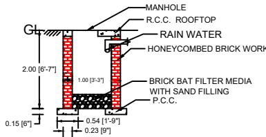
SECTION ON O - P
