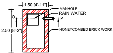
PLAN RAIN WATER HARVESTING
