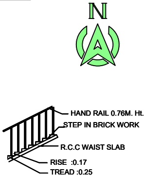
STAIR CASE DETAIL
