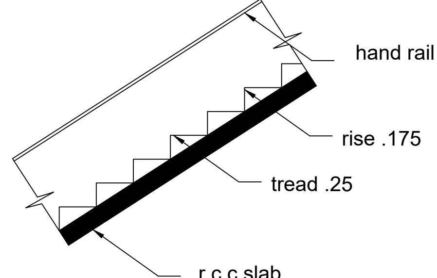
STAIR
