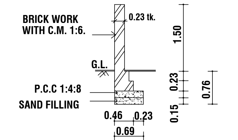
SECTION OF COMPOUND WALL
