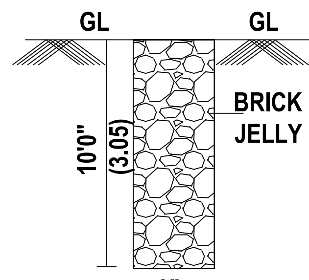
PERCULATION PIT
