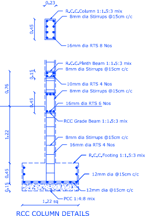
RCC COLUMN DETAILS
