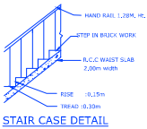
STAIR CASE DETAIL
