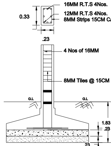
RCC COLUMN DETAILS
