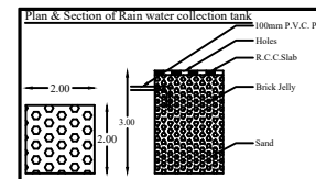
Plan & Section of Rain water collection tank
