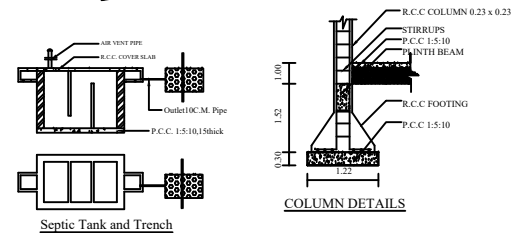
Septic Tank and Trench
