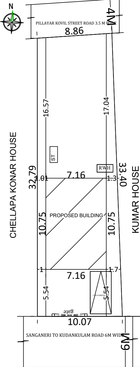
SITE PLAN 1:200 SCALE
