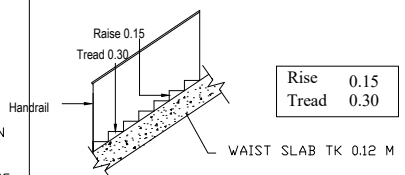
STAIRCASE DETAIL
