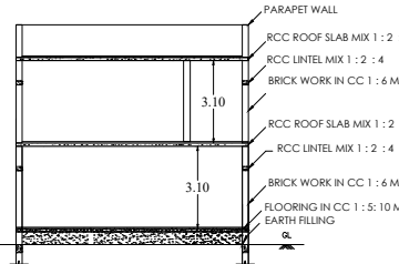
SECTION ON AB & ( HALF ELEVATION)
