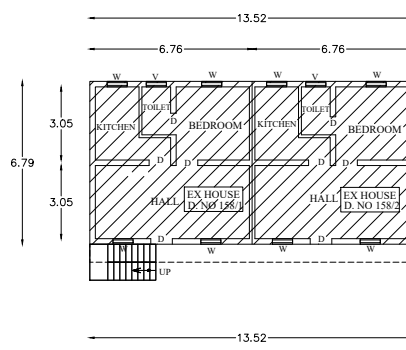
EX GROUND FLOOR PLAN
