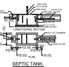
SEPTIC TANK
