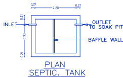
PLAN SEPTIC. TANK
