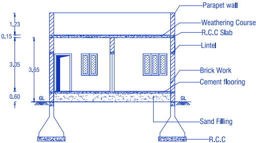
CROSS SECTION ON 'A-B'
