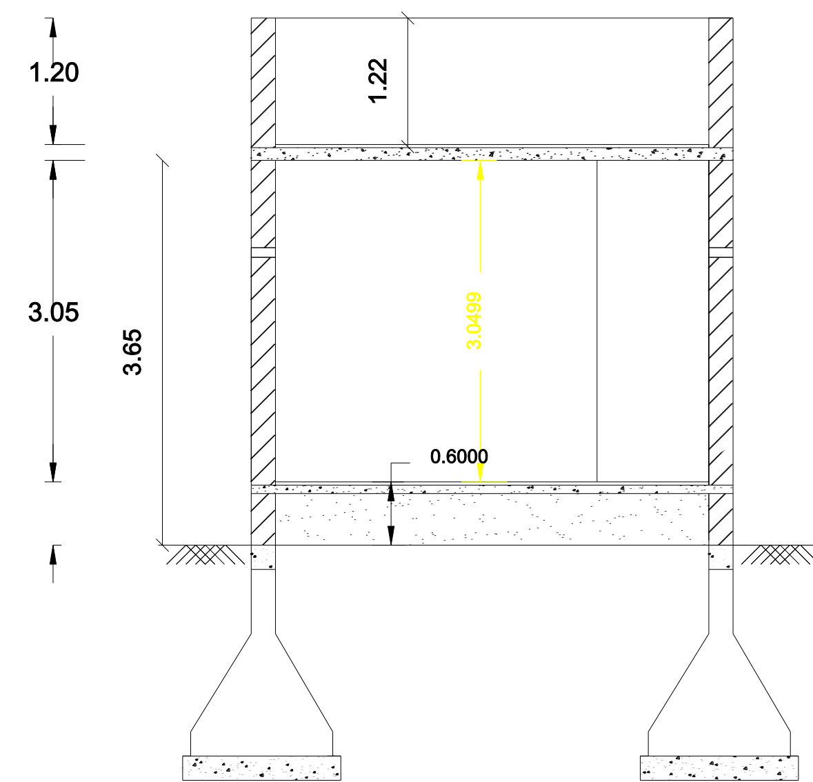
CROSS SECTION ON 'AB'
