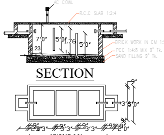
SECTION PLAN SEPTIC TANK DETAILS
