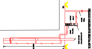
RAIN WATER HARVESTING SYSTEM
