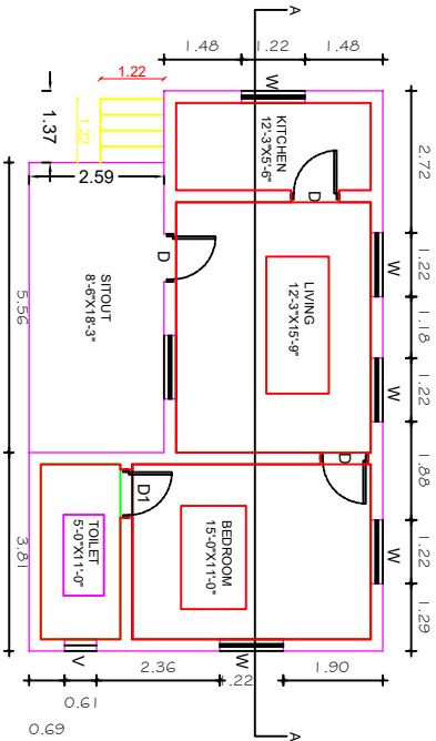
PLAN
