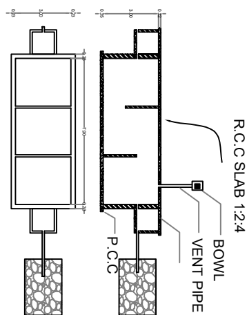
SEPTIC TANK AND TRENCH NTS
