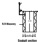
Soakpit section
