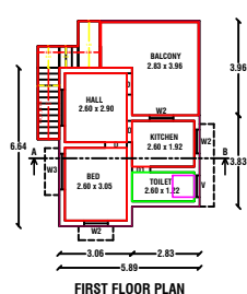
FIRST FLOOR PLAN SCALE 1:100
