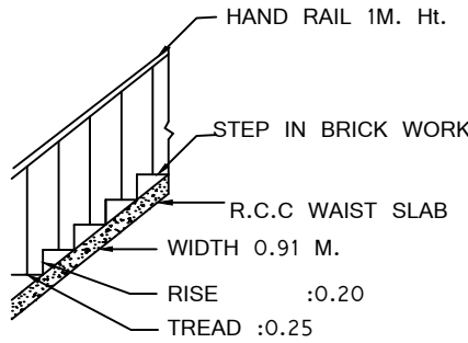
STAIR DETAIL
