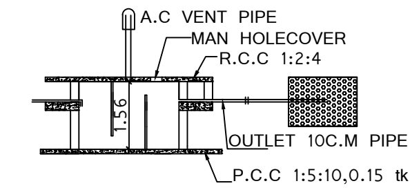
SECTION 0.2 2.34 0.2 0.2 0.38 0.38 PLAN OF SEPTIC TANK & TRENCH
