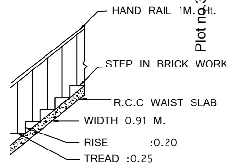
STAIR DETAIL
