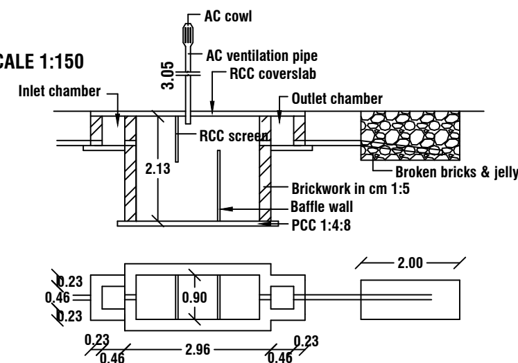
SEPTICTANK DETAILS
