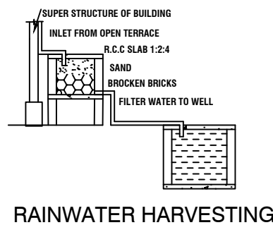
RAINWATER HARVESTING
