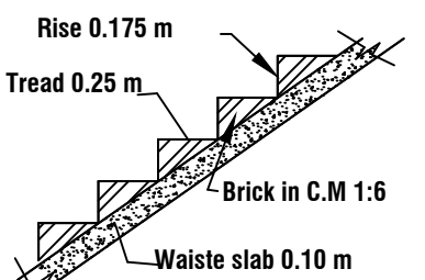
STAIR DETAILS
