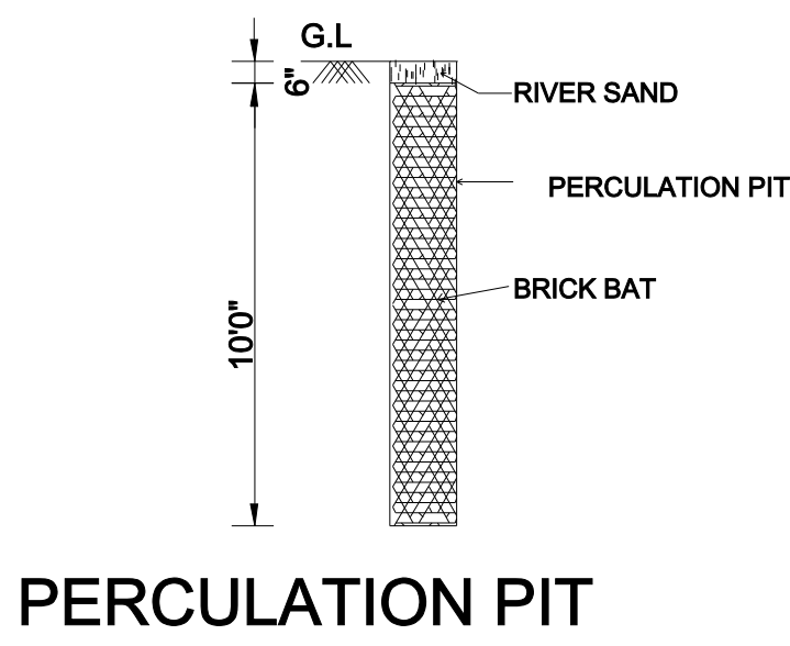
PERCOLATION PIT
